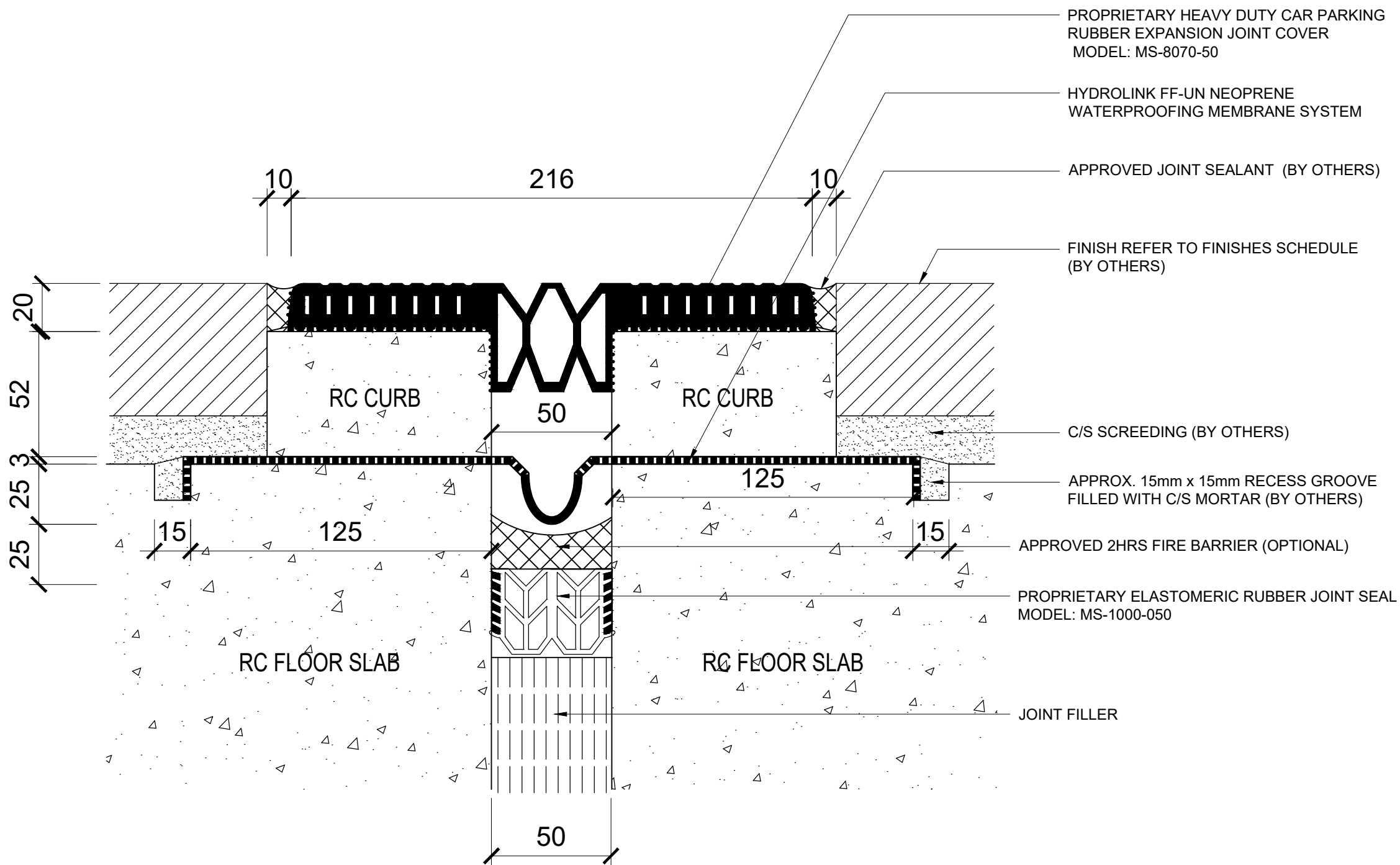
PROPRIETARY HEAVY DUTY MOVEMENT JOINT COVER MODEL NO.: HI-LINK MS-8070-50 (FLOOR TO FLOOR)
