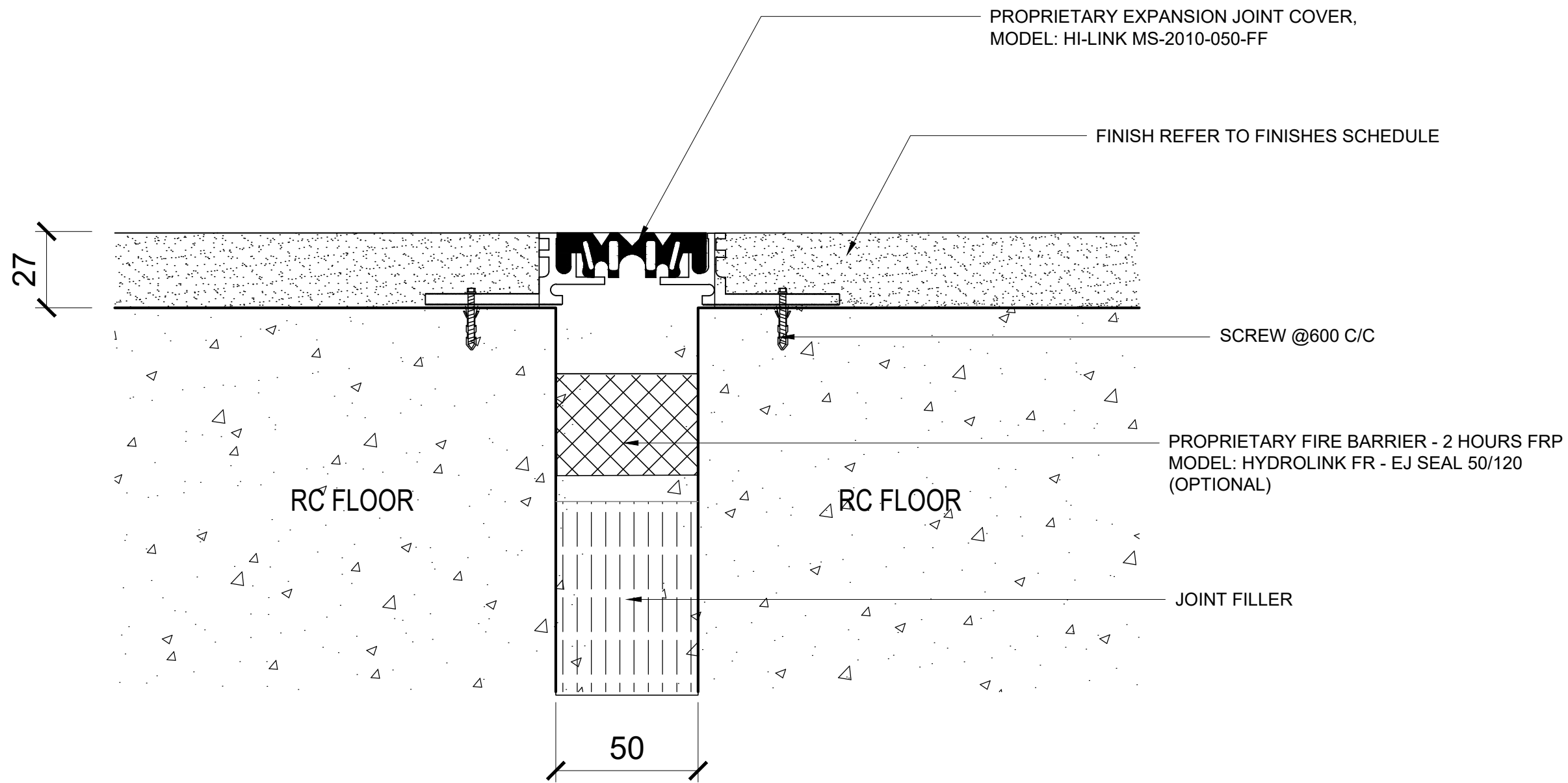
9 PROPRIETARY FLUSH TINE LINE MOVEMENT JOINT COVER DETAIL FOR INTERNAL FLOOR (FLOOR TO FLOOR)
