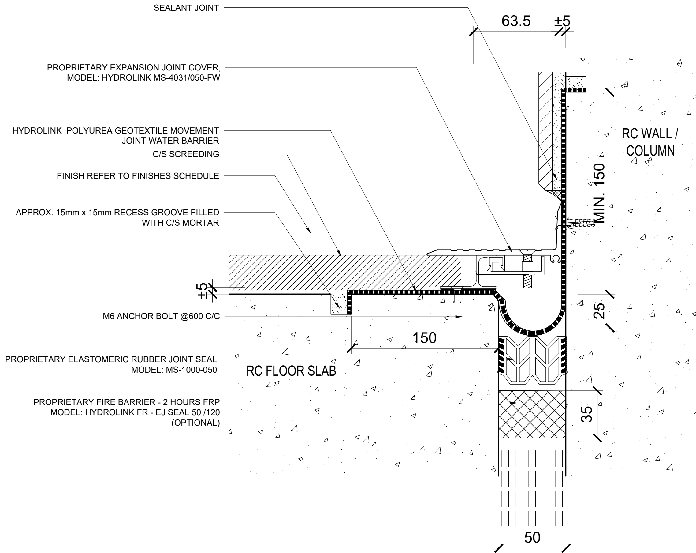
8 PROPRIETARY METAL MOVEMENT JOINT COVER DETAIL MODEL NO.: HI-LINK MS-4031-50 (FLOOR TO WALL)
