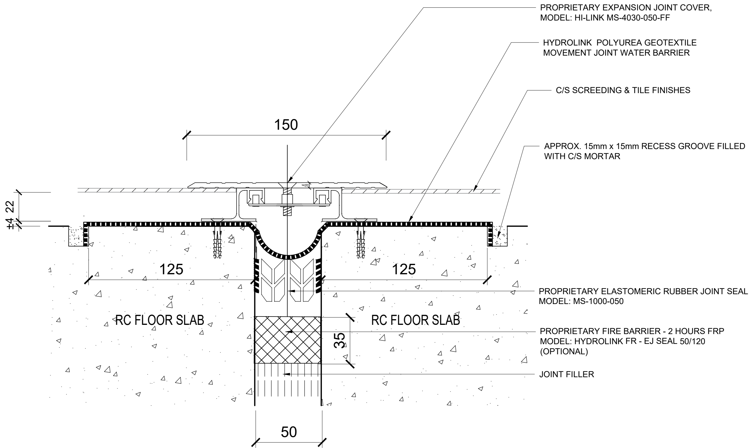
7 PROPRIETARY METAL MOVEMENT JOINT COVER DETAIL MODEL NO.: HI-LINK MS-4030-50 (FLOOR TO FLOOR)
