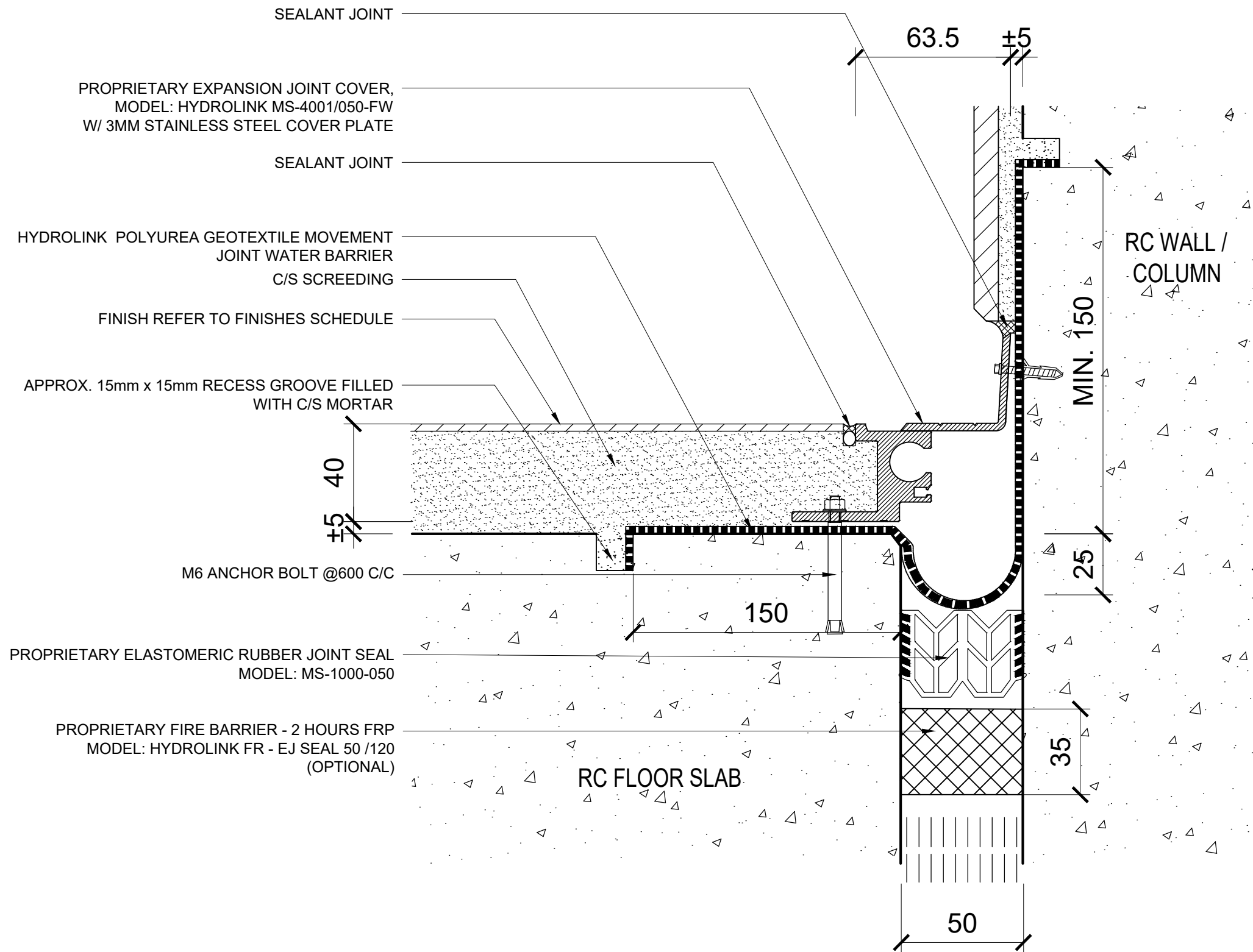
6 PROPRIETARY METAL MOVEMENT JOINT COVER DETAIL MODEL NO.: HI-LINK MS-4001-50 (FLOOR TO WALL)
