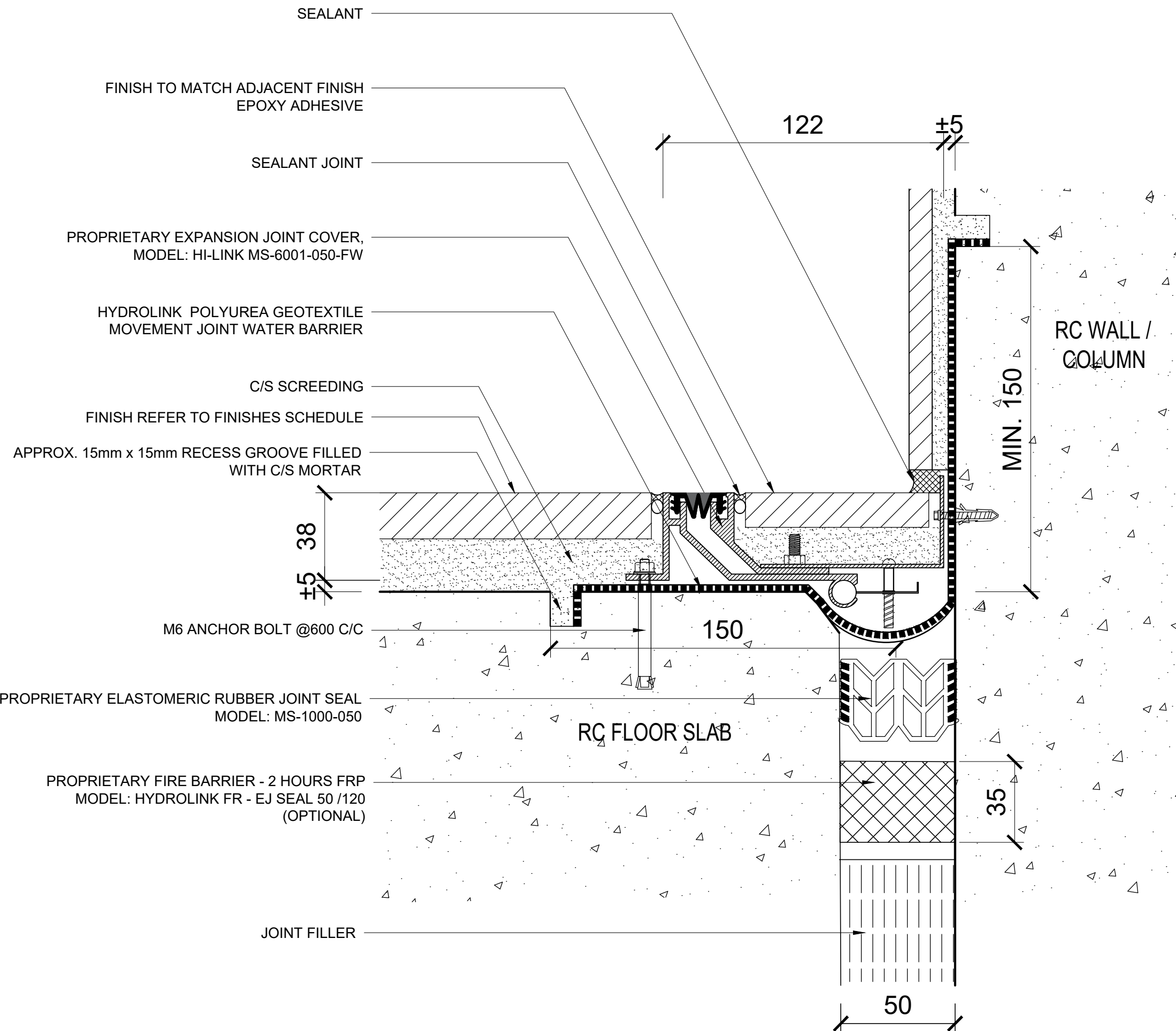
2 PROPRIETARY ALUMINUM MATCHING COVER MOVEMENT JOINT SYSTEM MODEL: HI-LINK MS-6001-50 (FLOOR TO WALL)
