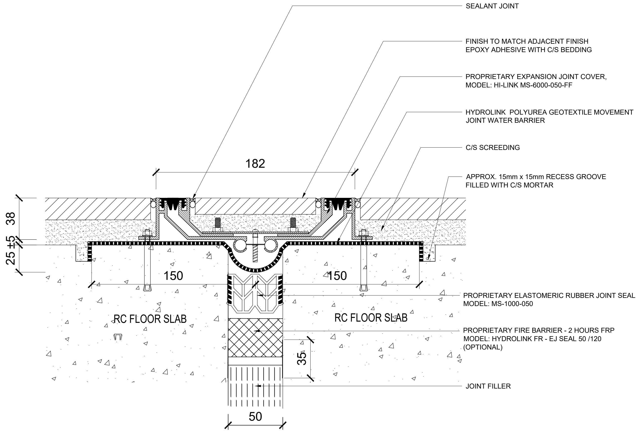
1 PROPRIETARY ALUMINUM MATCHING COVER MOVEMENT JOINT SYSTEM MODEL: HI-LINK MS-6000-50(FLOOR TO FLOOR)
