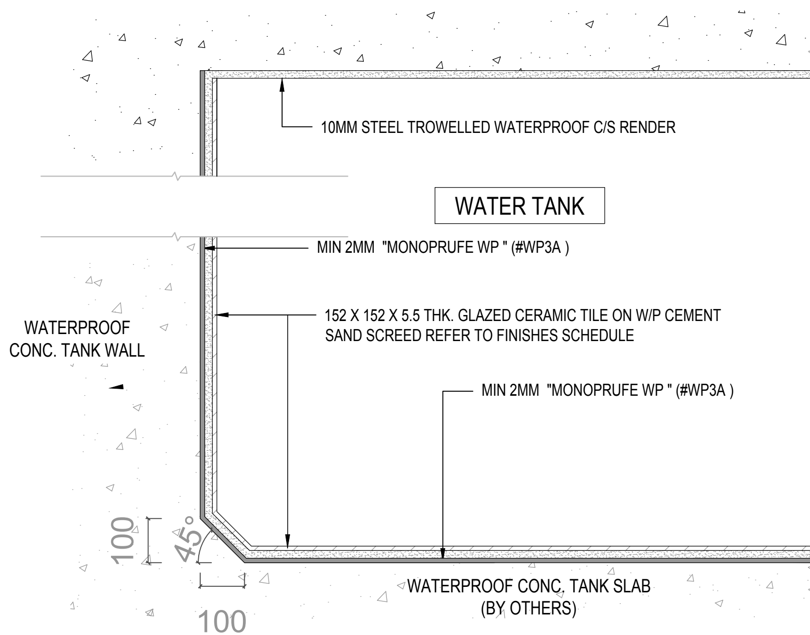
01 TYPICAL WATERPROOFING DETAIL FOR SPRINKLER WATER TANK, F.S. WATER TANK, FLUSH WATER TANK
