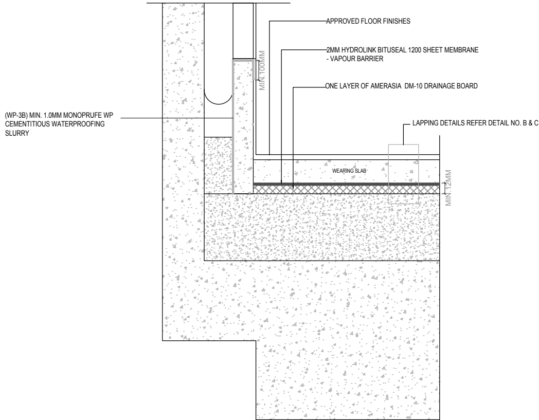
A VAPOUR BARRIER DETAIL FOR BASEMENT Scale:
