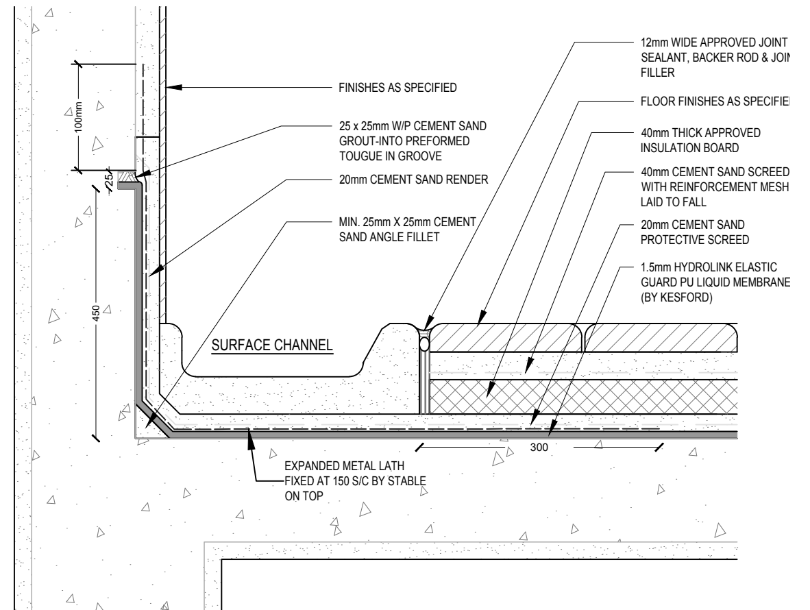
B WATERPROOFING DETAIL FOR FLOOR WITH SURFACE CHANNEL
