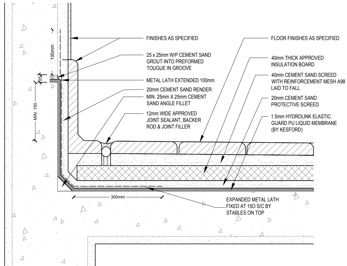
A WATERPROOFING DETAIL FOR FLOOR
