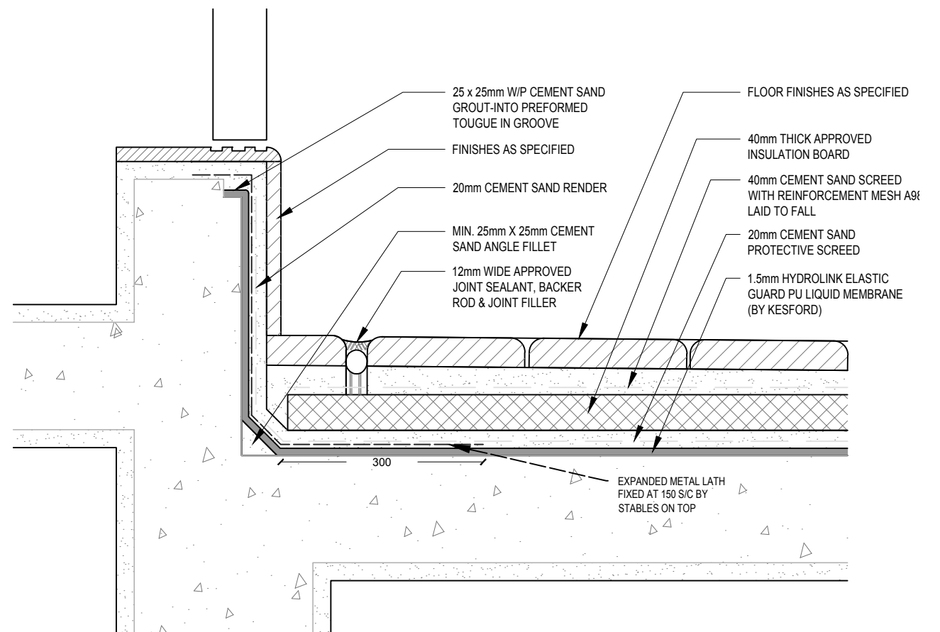
D WATERPROOFING DETAIL FOR PLINTH / KERB AREA
