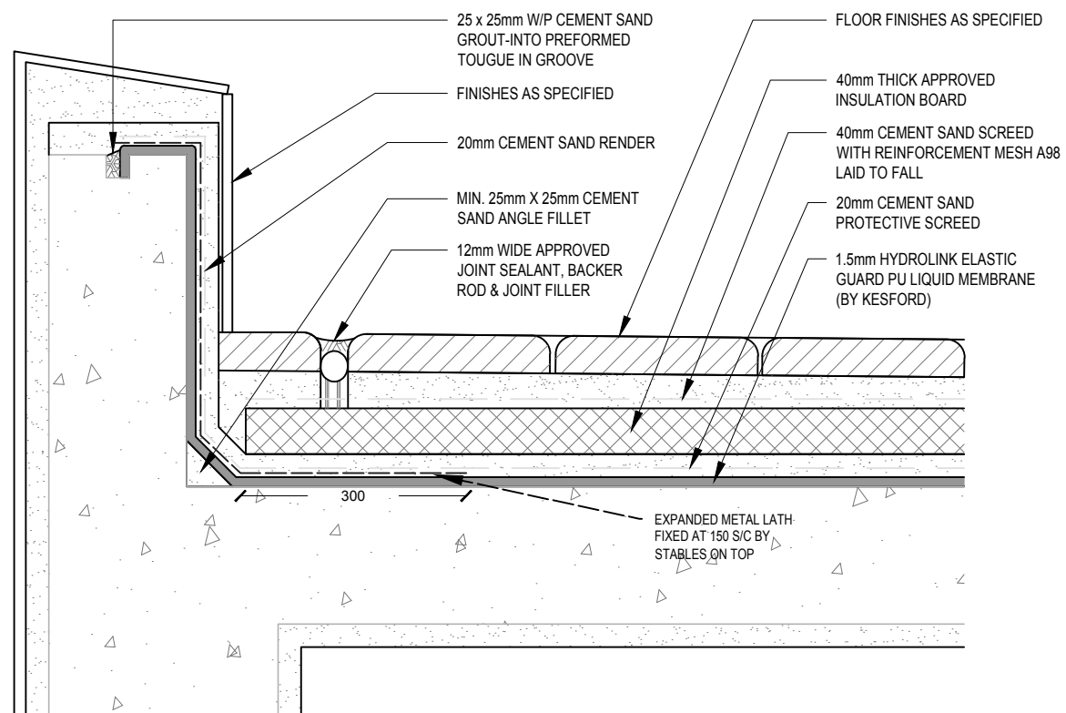
C WATERPROOFING DETAIL FOR PLINTH / KERB AREA
